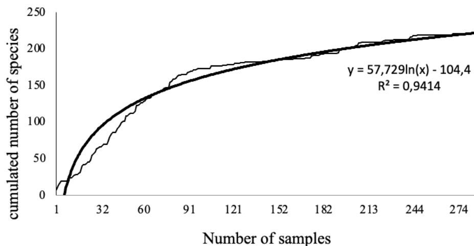
Figure 2: Species accumulation and rarefaction curve
