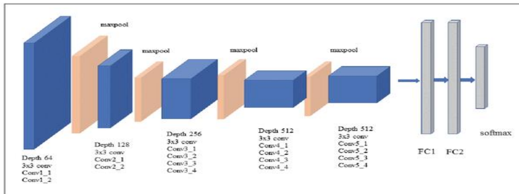
Figure 3: VGG19 architecture[12]
