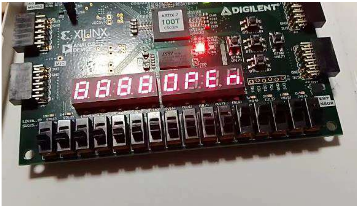
Fig.6: Hardware implementation
