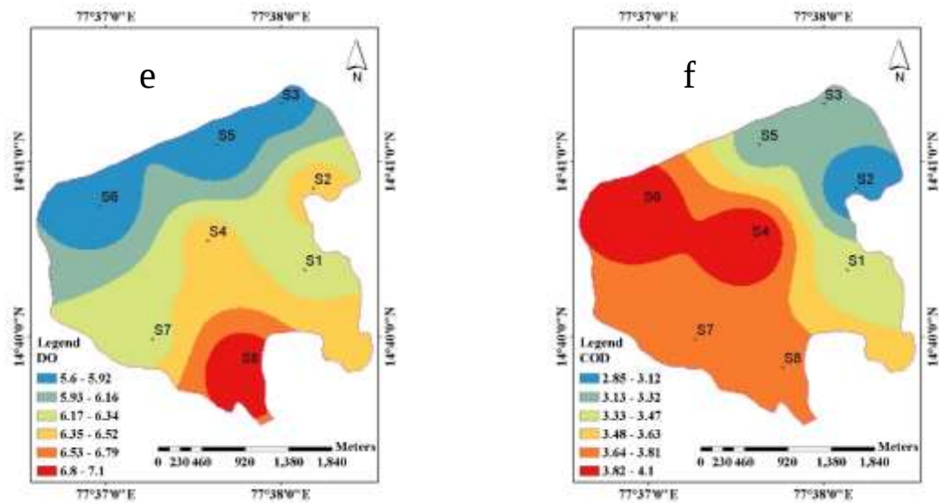
Fig. 3. Spatial behaviour of (a) pH, (b) Temperature, (c) EC, (d) TDS, (e) DO and (f) COD.
