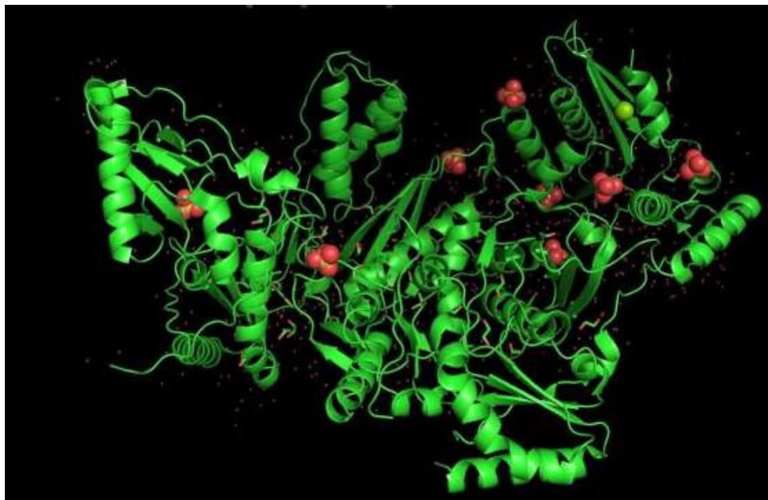
Figure. 2 The crystal structures of K103N/Y181C mutant RT (PDB ID: 6C0R) In Figure.3 the crystallography of the wild-type HIV-1 RT (PDB ID: 6C0J) K103N/Y181C mutant RT (PDB ID: 6C0R) are superimposed for further docking interactions with drugs.
