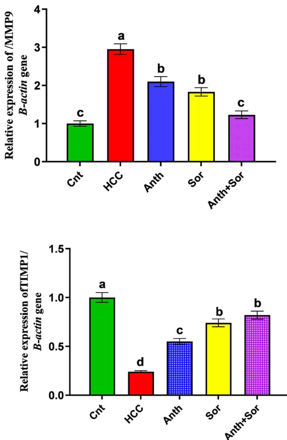
Figure (3): Effect of ANTH and/or SOR on metastasis-related genes (MMP9, TIMP1). Normal control (Cnt), HCC, HCC treated by (ANTH), HCC treated by (SOR), and HCC treated by ANTH and SOR (ANTH+SOR) rats. Values are expressed as mean \pm SEM ( n = 7 ). Values carrying different lower case letter are significantly different at P < 0.05 .
