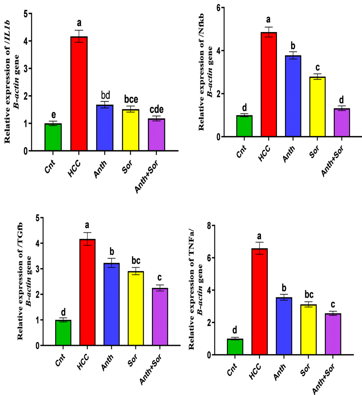
Figure (2): Effect of ANTH and/or SOR on the relative expression of inflammation-related genes IL1b, NF-kB TGF-β and TNF-α genes. Normal control (Cnt), HCC, HCC treated by (ANTH), HCC treated by (SOR), and HCC treated by ANTH and SOR (ANTH+SOR) rats. Values are expressed as mean ± SEM (n = 7). Values carrying different lower case letter are significantly different at P < 0.05 .
