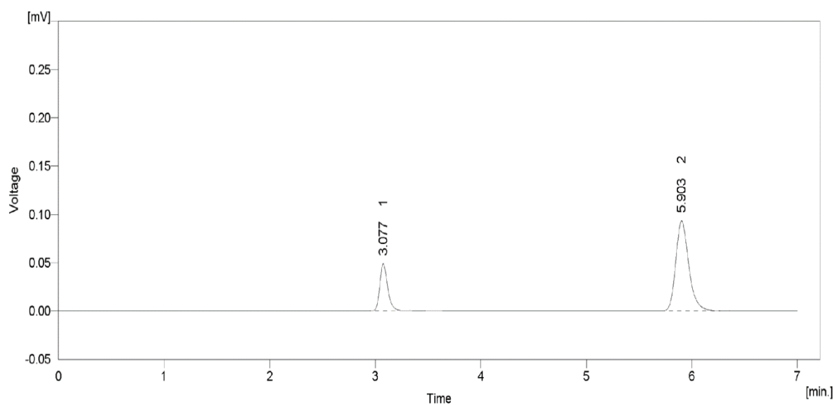
Fig 10: Chromatogram of Dexamethasone (IS,10 \mu g/ml) and Dutasteride(50 \mu g/ml)
