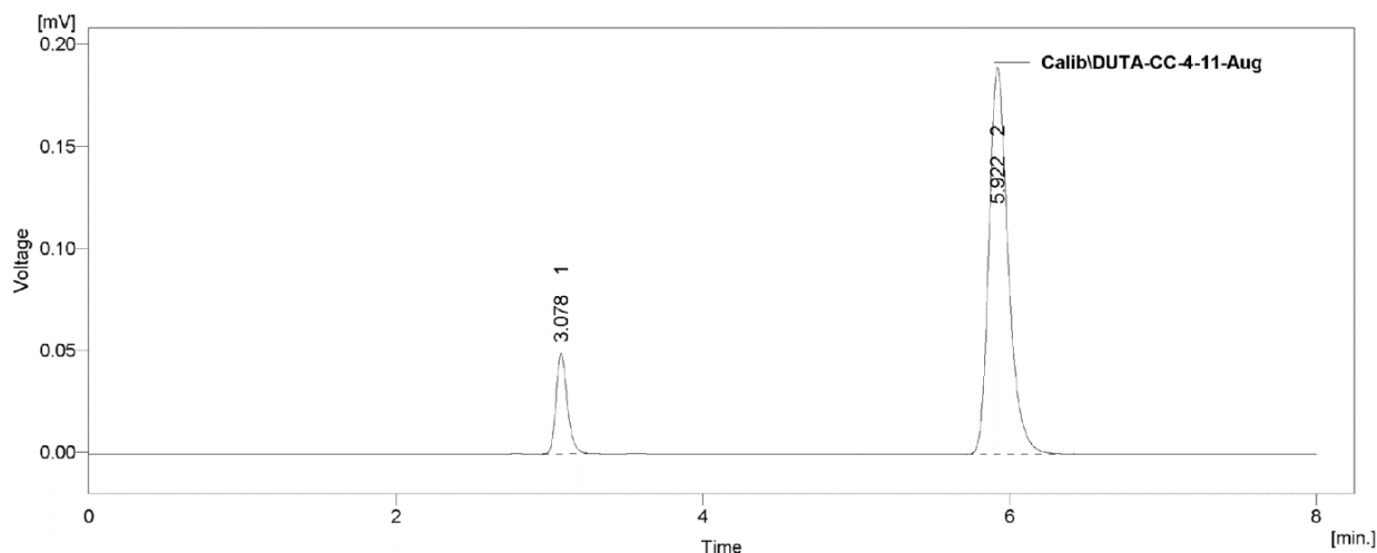
Fig 8: Chromatogram of Dexamethasone (IS, 10µg/ml) and Dutasteride(100µg/ml)
