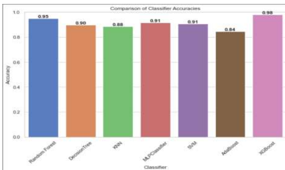
Fig. 6. Comparative Analysis of Model Accuracies
