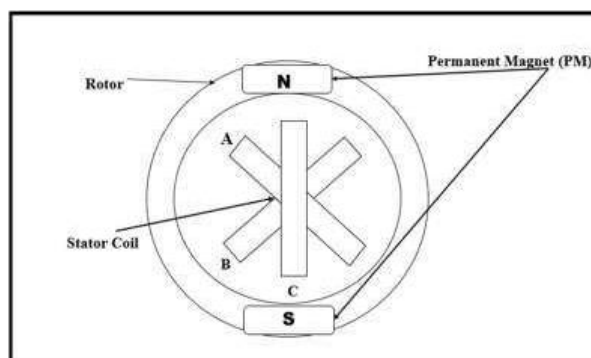
Fig -9: Out-runner type BLDC Motor
