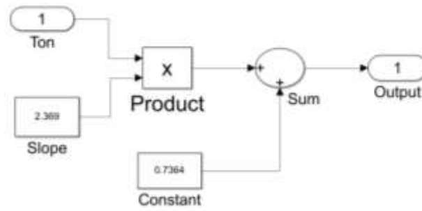
Figure.6 Simulation design of pH system block
