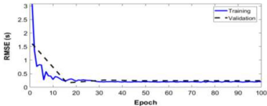
Figure 11. Training and validation performance of LSTM to predict T_{on\_pH} of buffer solution pump
