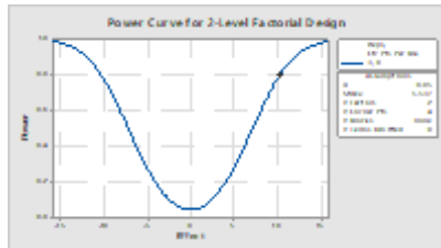
Fig 1 Power curve
