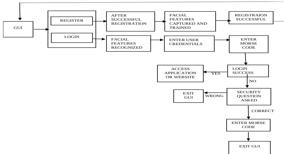
Fig. 1. System Architecture
