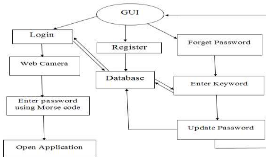
Fig. 3. Dataflow diagram
