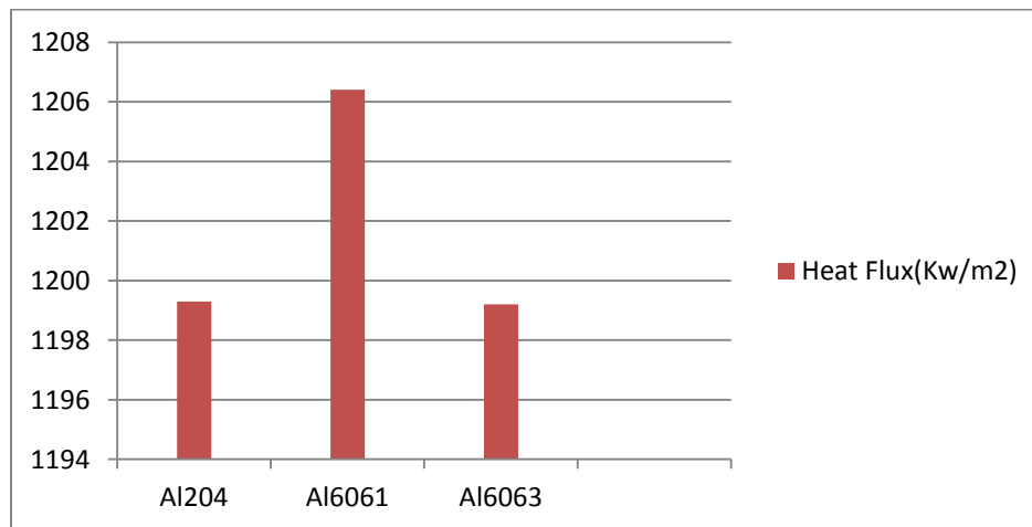
Figure 13: Maximum heat flux for Al Alloy Fins
