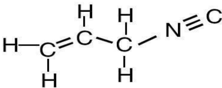
Allyl isocyanide
