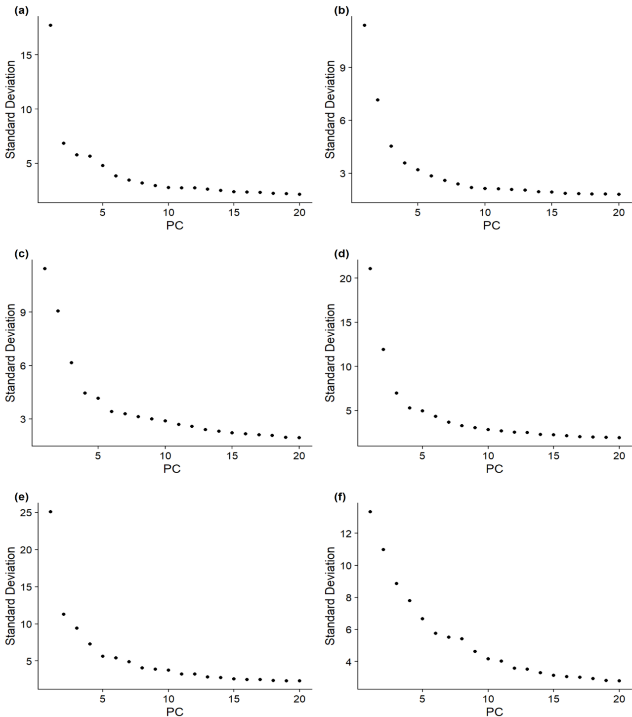
Fig.2: Elbow plots showing PC wise standard deviations present in the datasets. (a) Breast cancer Dataset 1 (b) Breast cancer Dataset 2 (c) Breast cancer Dataset 3 (d) Lung cancer Dataset 1 (e) Lung cancer Dataset 2 (f) Lung cancer Dataset 3
