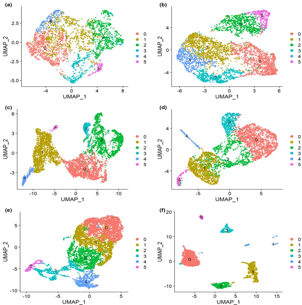
Fig.4: Plots showing six different clusters obtained after performing UMAP in the datasets. (a) Breast cancer Dataset 1 (b) Breast cancer Dataset 2 (c) Breast cancer Dataset 3 (d) Lung cancer Dataset 1 (e) Lung cancer Dataset 2 (f) Lung cancer Dataset 3
