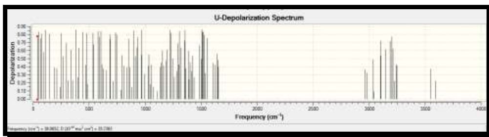
Figure 5. IR Spectrum of Norclozapine
